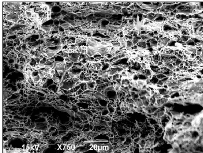
Figure 11: Example of ductile fracture under SEM (Ziemian, Constance & Sharma, Mala & Whaley, Donald, 2012)
