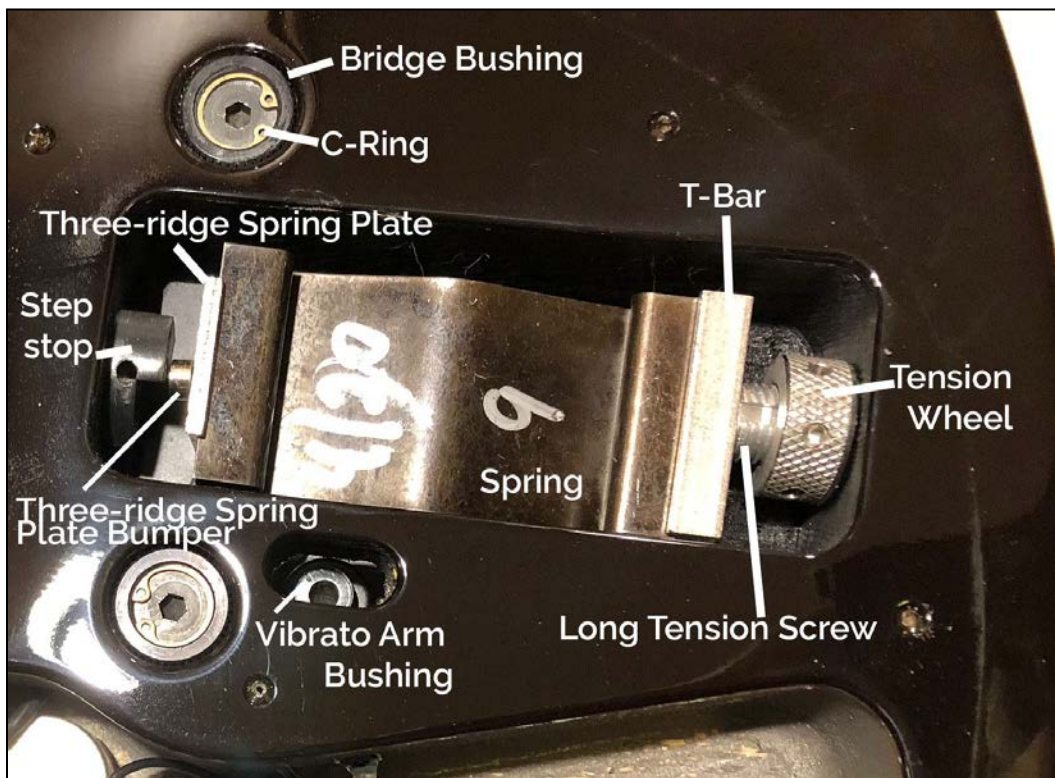
Figure 1: Spring system in a Parker Fly guitar (Courtesy of Professor Manzo)
