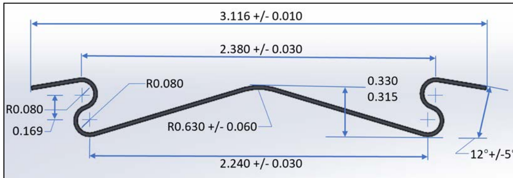
Figure 14: SolidWorks model of 9 gauge flat spring with dimensions
