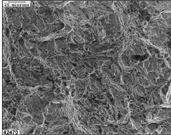
Figure 12: Example of brittle fracture under SEM (Bahrami, Amir & Zhang, Yanhui & PeterTubby, 2015)
