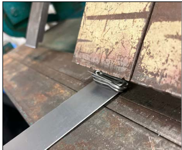
Figure 36: Sheet metal with spacer for second bend
