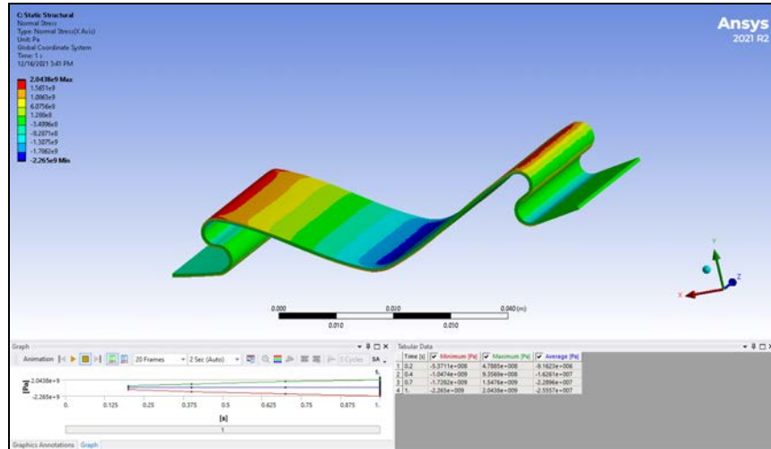
Figure 16: Ansys model for stress analysis
