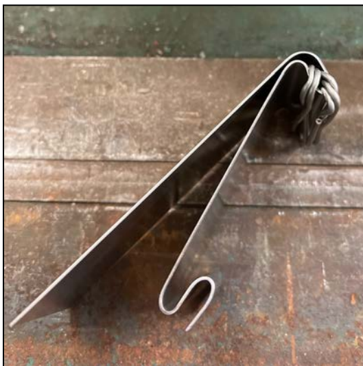
Figure 40: Flat spring with excess material and spacer
