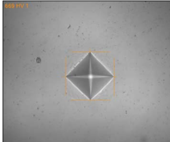
Figure 25: Hardness Testing using a Vickers indenter
