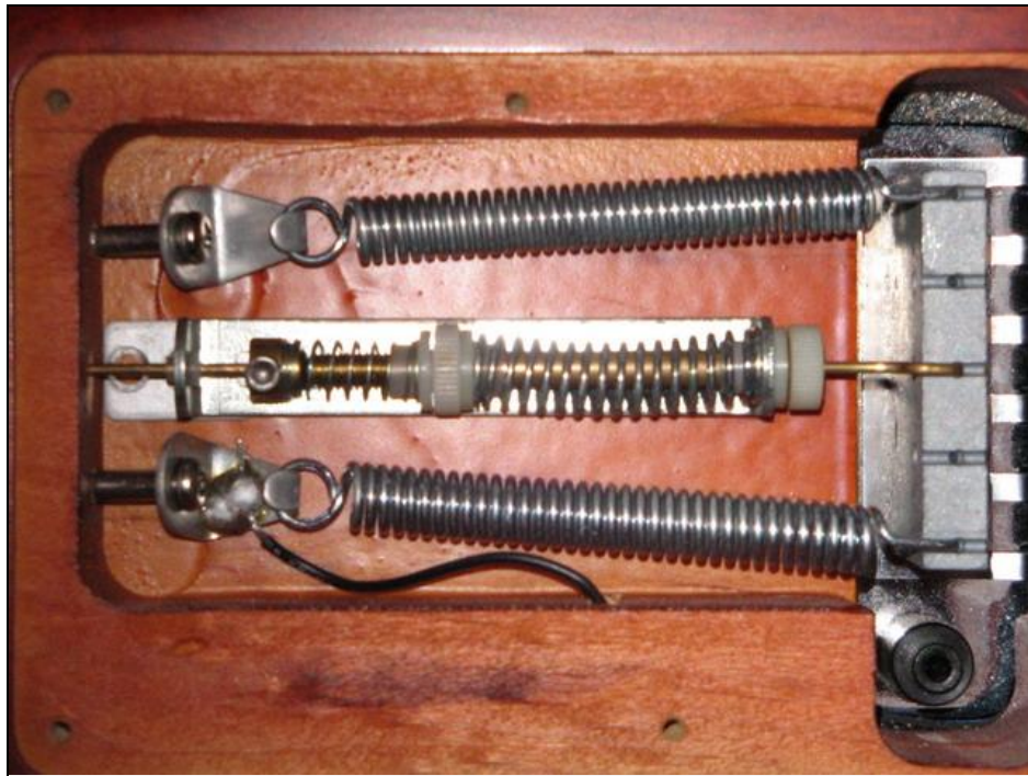
Figure 4: The Hipshot Tremsetter stabilizer replaces the central spiral extension spring
