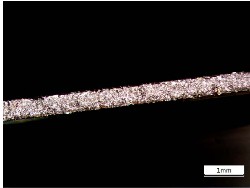
Figure 19: Image of fracture surface from optical stereo microscope
