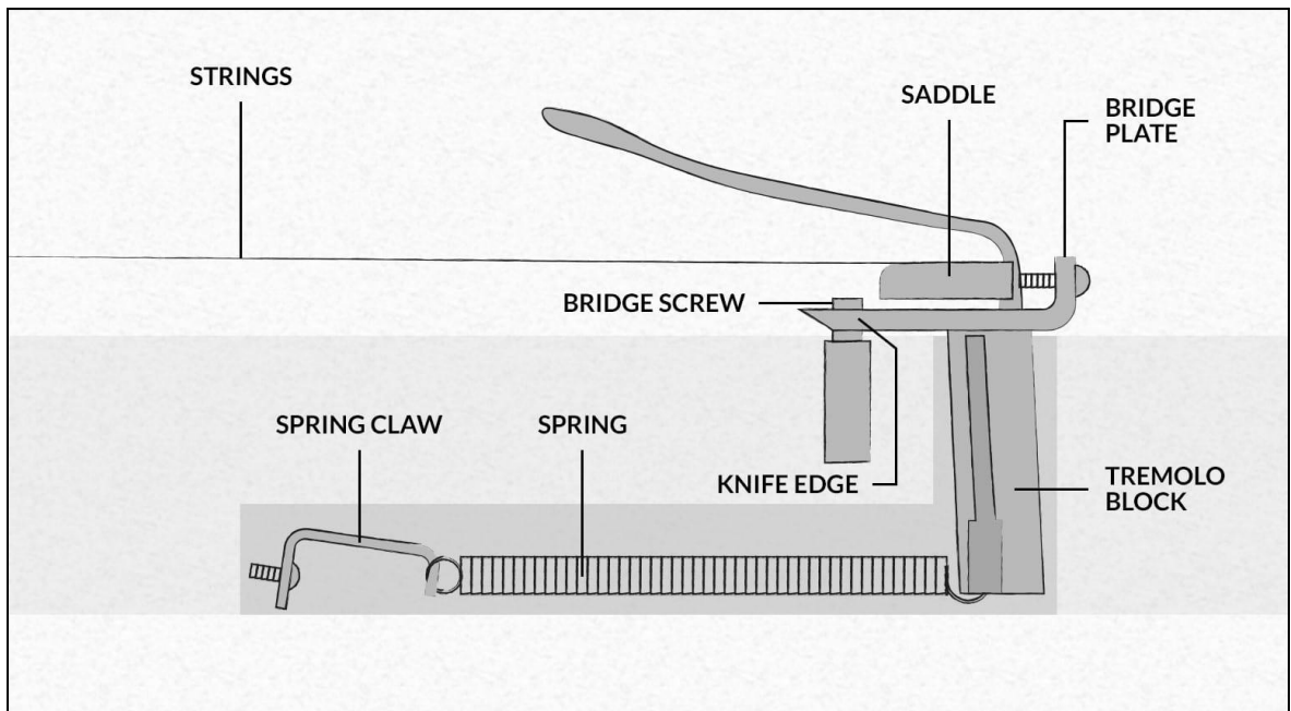
Figure 3: Diagram of the entire typical vibrato system
