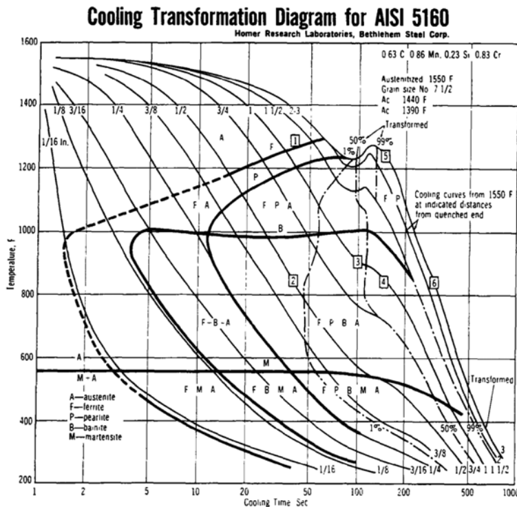
Figure 9: Cooling transformation diagram for AISI 5160 (AISI 5160 (High Strength Machinery Steel), 1952)
