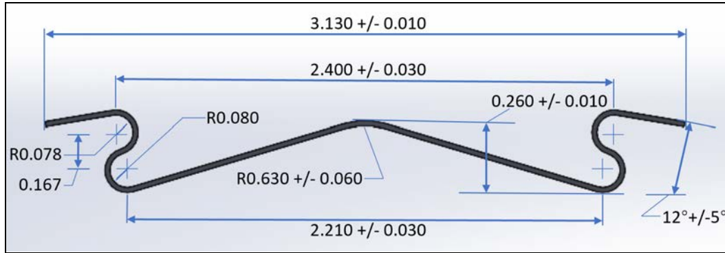
Figure 15: SolidWorks model of 10 gauge flat spring with dimensions
