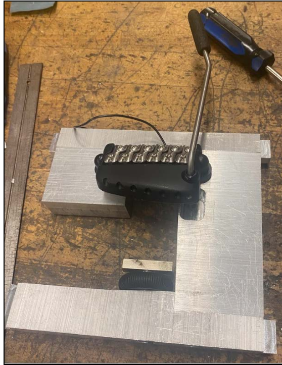
Figure 48: Image of assembled 6061 Aluminum Rig
