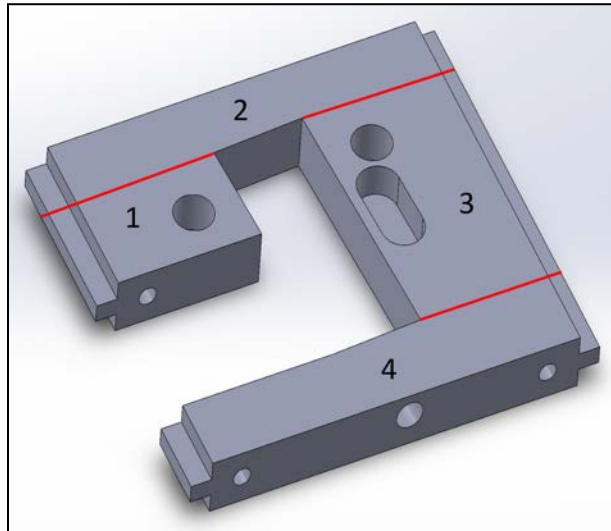
Figure 44: SolidWorks model of rig broken down into four pieces for assembly
