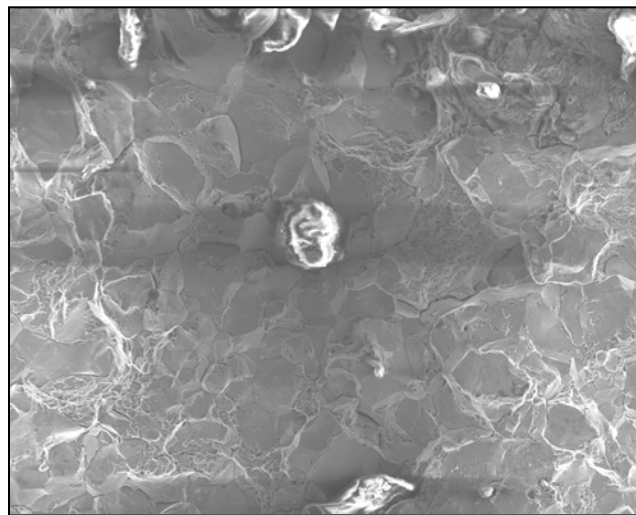
Figure 20: Image of fracture surface showing inclusion and brittle fracture
