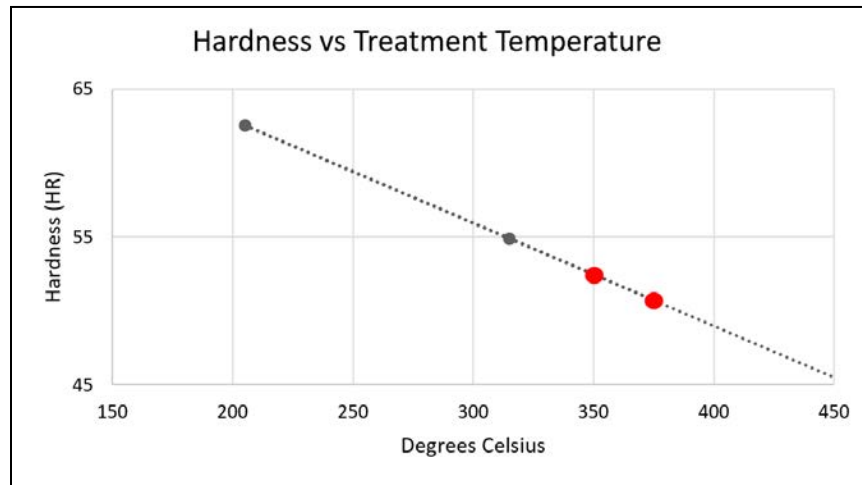
Figure 27: Hardness vs. Heat Treatment Temperature Graph
