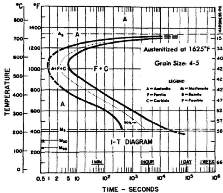
Fig. 1 — Isothermal-transformation diagram of AISI 1095 containing 0.89% carbon and 0.29% manganese.
