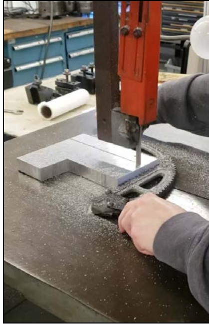
Figure 46: Contouring the block of Aluminum
